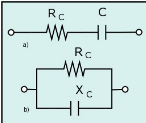
Two equivalent circuits of a real capacitor
